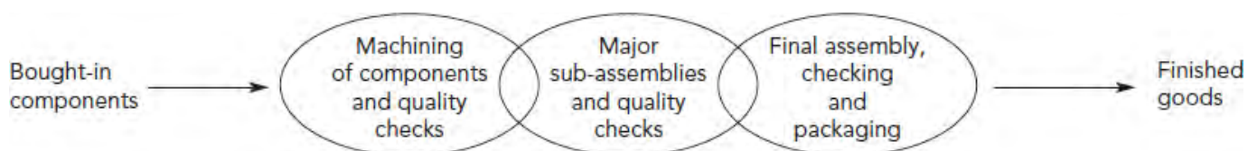
Figure 28.8: How cell production might be organised in an assembly plant
