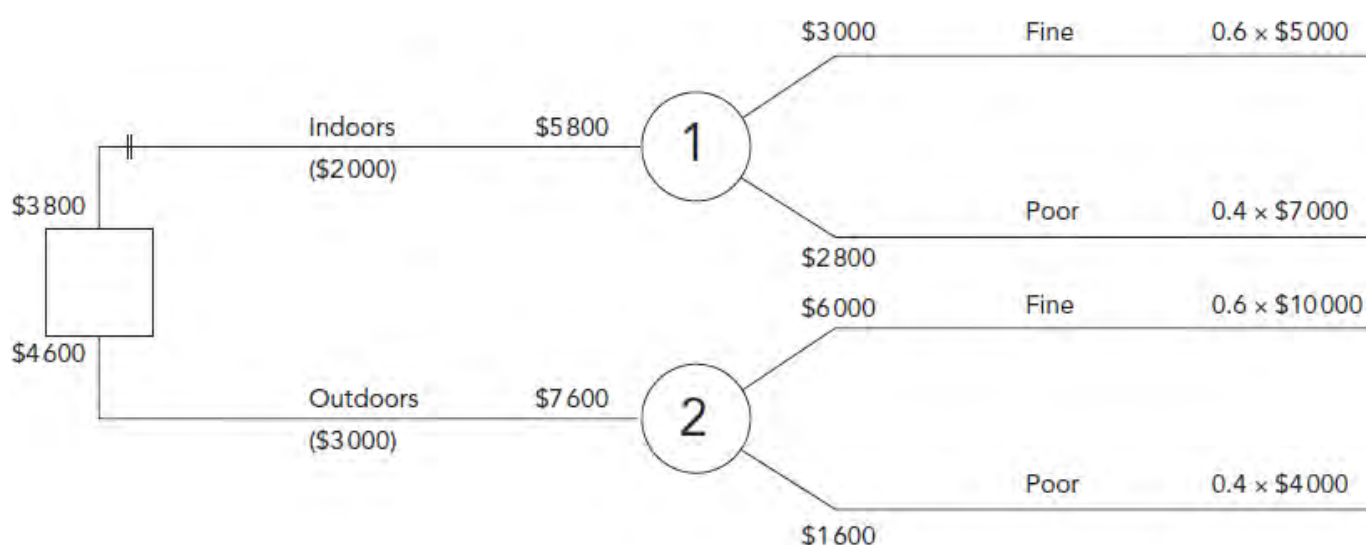
Figure 8.10: Calculating expected values, working from right to left
